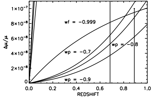
Fig. 6. This is an expanded view of the late time \mu evolution shown in Figure 5 to show the detail of the \Delta\mu/\mu near the most restrictive constraint at z = 0.88582 .
