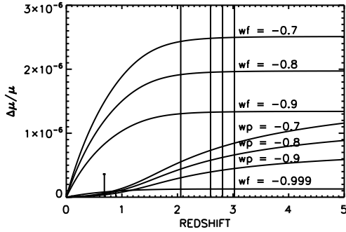
Fig. 5. Values of \Delta\mu/\mu versus redshift for Model 1 with the future, wf , and past, wp , values labeled on the plot. The plots labeled with wf values are the thawing models shown in figure 4 and those labeled with wp values are the freezing models.
