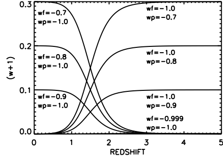
Fig. 4. Values of (w + 1) versus redshift for Model 1 with the future, w_f , and past, w_p , values labeled on the plot. Note that the thawing model with w = 0.999 has a future (w + 1) value of 0.001 which is not visible on the scale of this plot. All of the cases have \tau = 0.1 and a_t = 0.4 .
