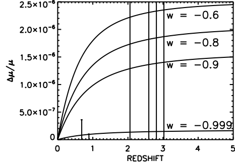
Fig. 2. Values of \Delta\mu/\mu versus redshift for constant value EoS models with the values labeled in the plot. In this and subsequent plots we leave in the higher redshift constraints even though they are off scale just to show that they are met.
