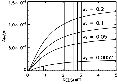
Fig. 3. Values of \Delta\mu/\mu versus redshift for w_0 = -1 and varying w_1 . The values of w_1 are labeled in the plot.
